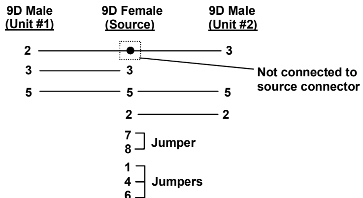
Figure 7- Pinout of Matrix-Y-1 cable
